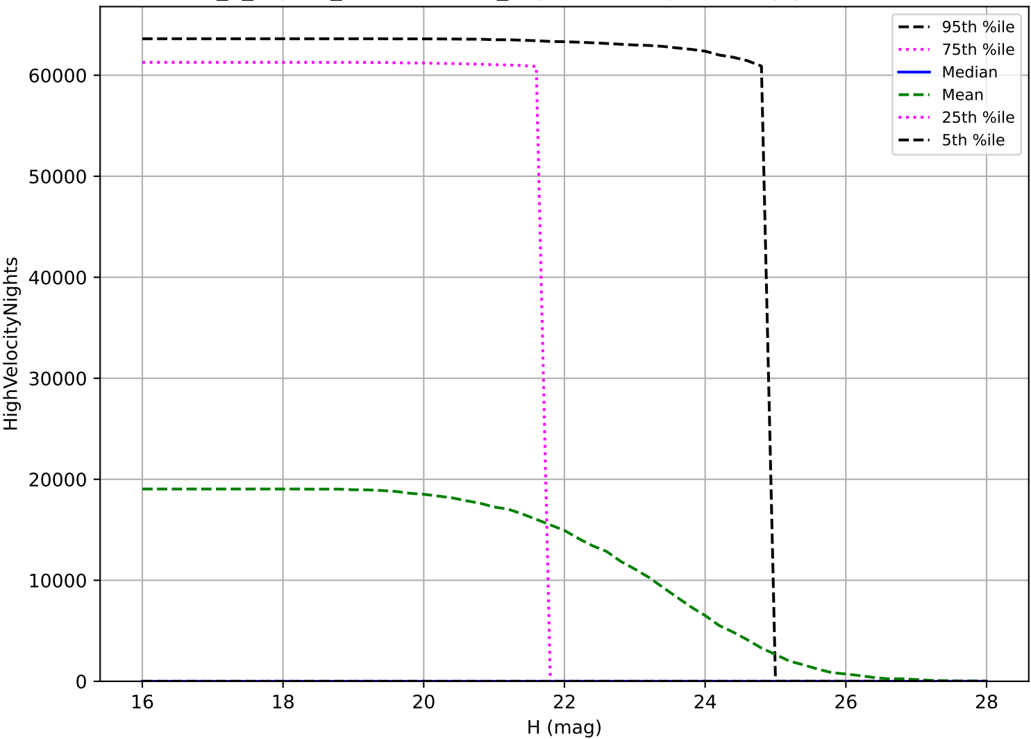
internal_u_expt30_nscale1.5v3.4_10yrs: NEO High velocity pair detection loss
