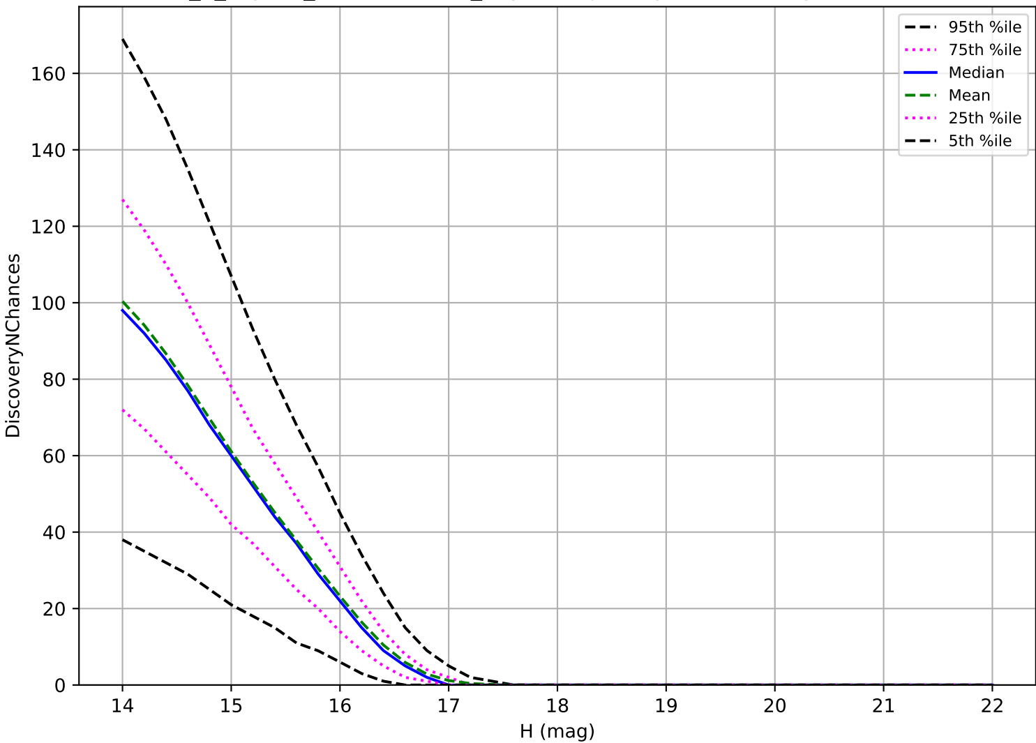
internal_u_expt30_nscale1.5v3.4_10yrs: Trojan 3 pairs in 15 nights detection loss
