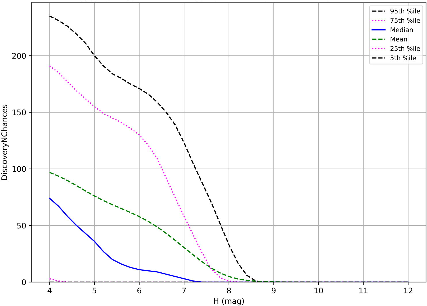
internal_u_expt30_nscale1.5v3.4_10yrs: TNO 3 pairs in 15 nights detection loss
