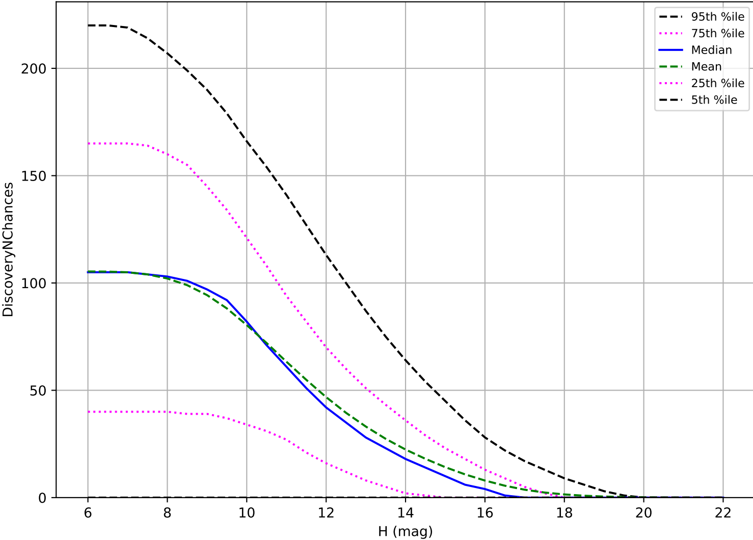
internal_u_expt30_nscale1.5v3.4_10yrs: OCC_r5 3 pairs in 15 nights detection loss
