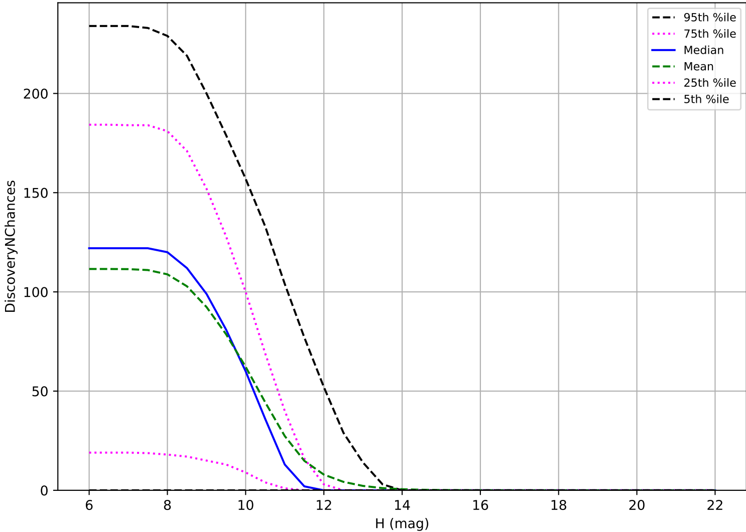
internal_u_expt30_nscale1.5v3.4_10yrs: OCC_r20 3 pairs in 15 nights detection loss
