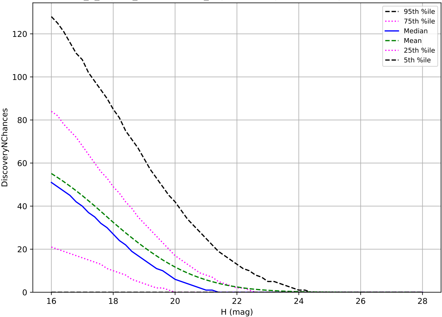
internal_u_expt30_nscale1.5v3.4_10yrs: NEO 3 pairs in 15 nights detection loss
