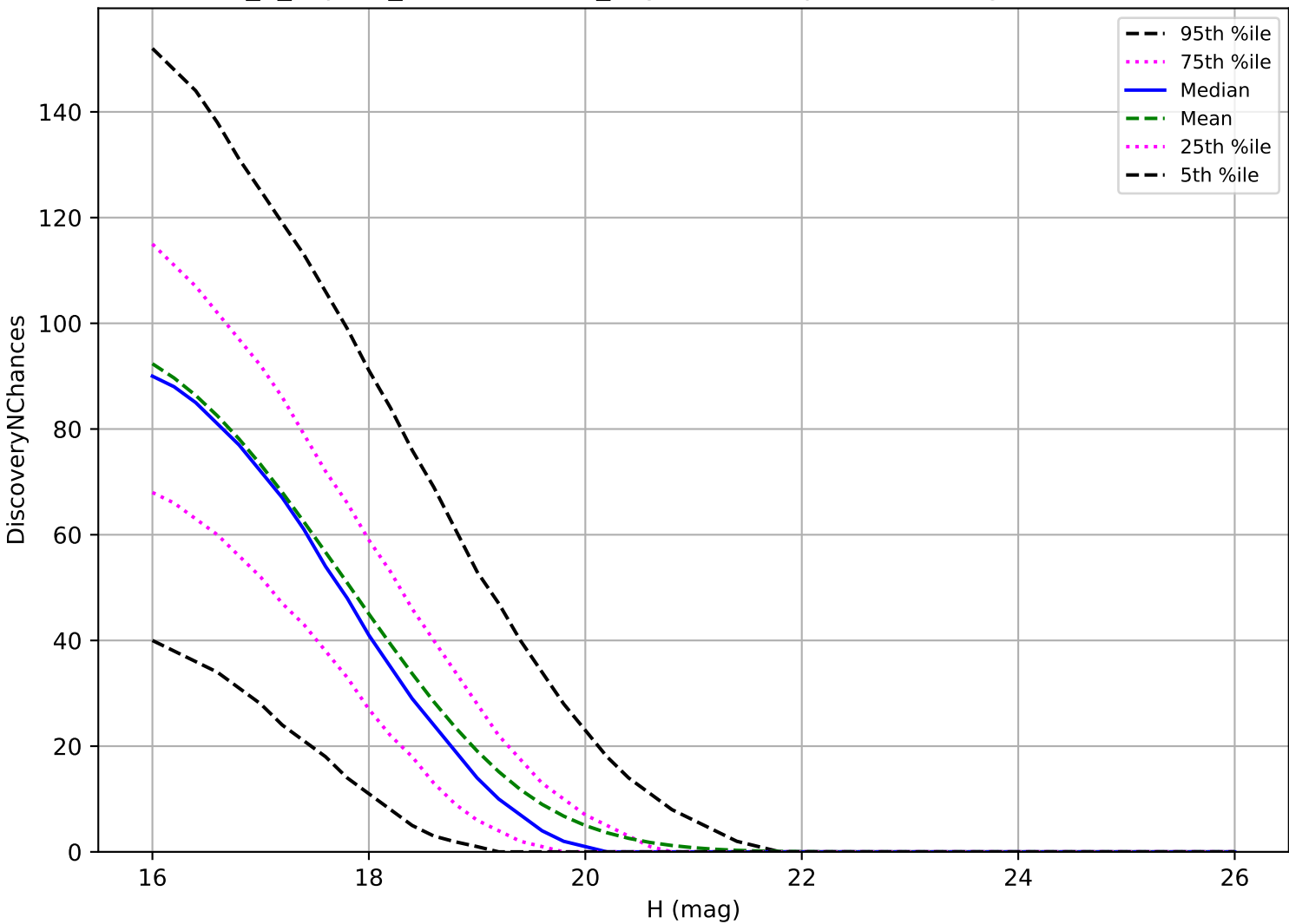
internal_u_expt30_nscale1.5v3.4_10yrs: MBA 3 pairs in 15 nights detection loss
