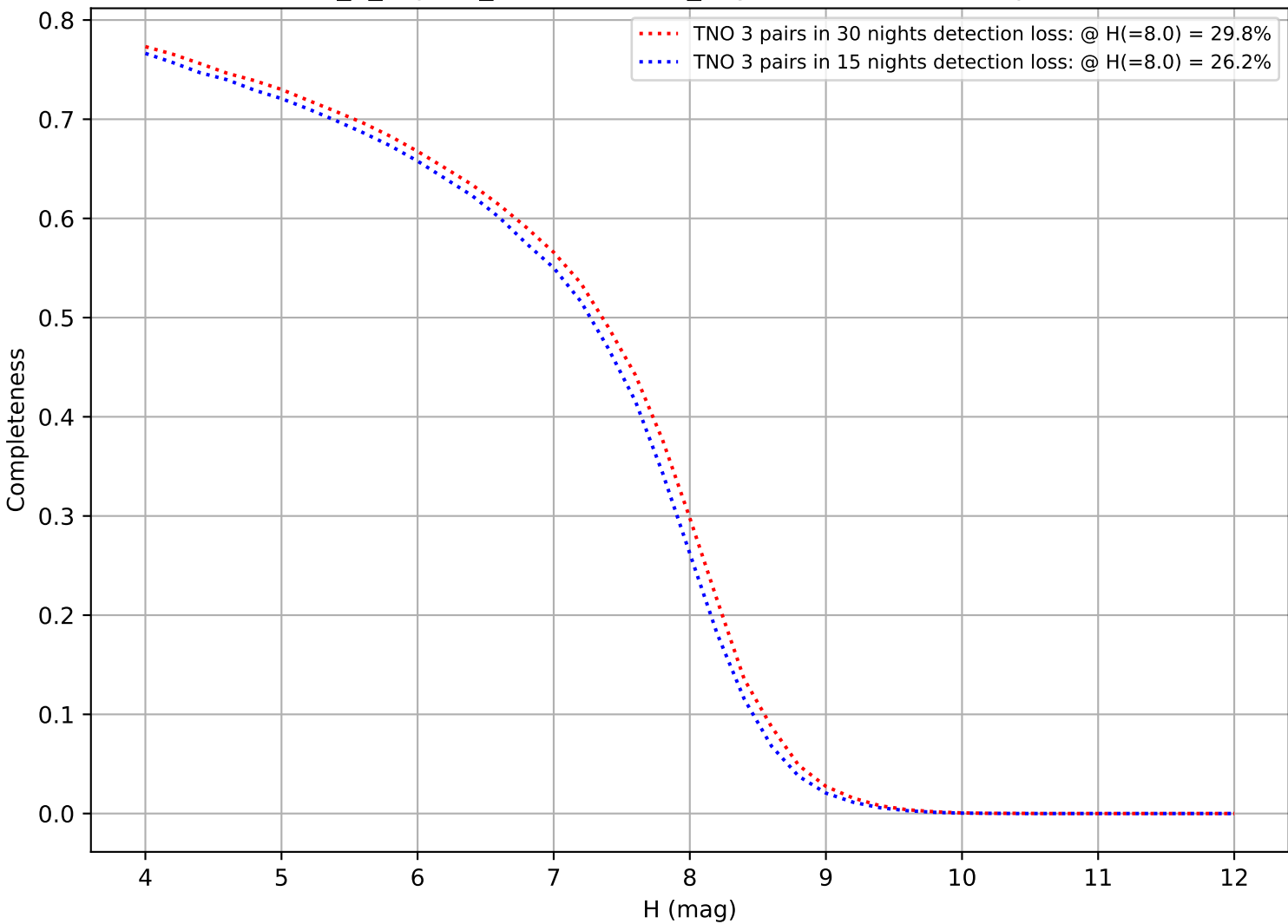
internal_u_expt30_nscale1.5v3.4_10yrs: DifferentialCompleteness
