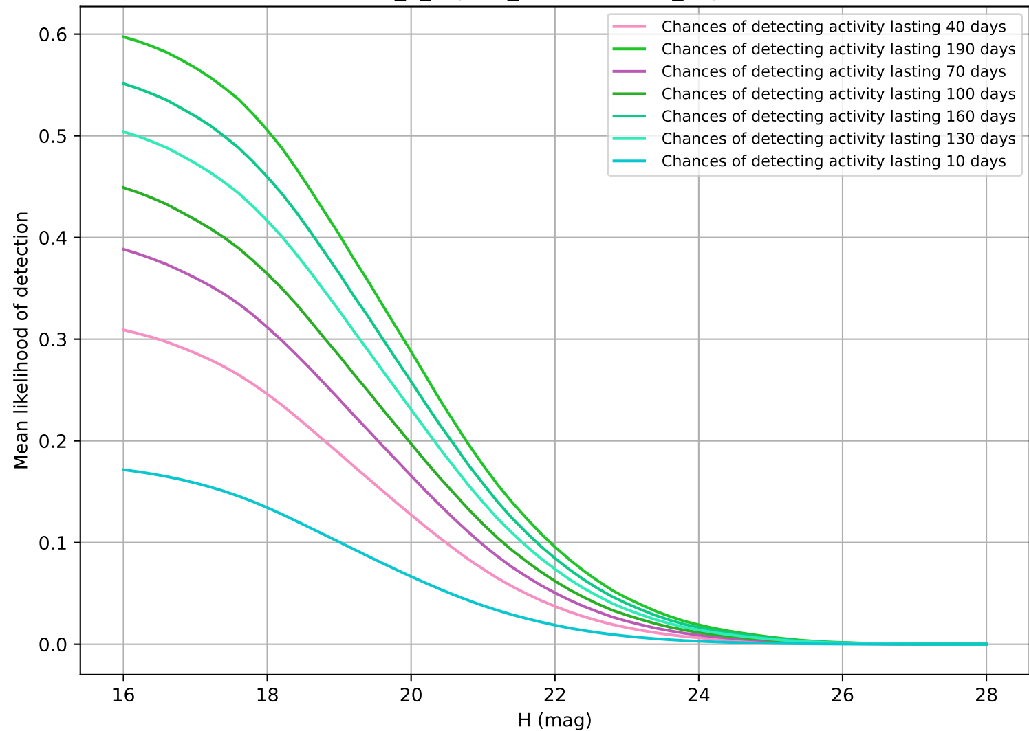
internal_u_expt30_nscale1.5v3.4_10yrs NEO
