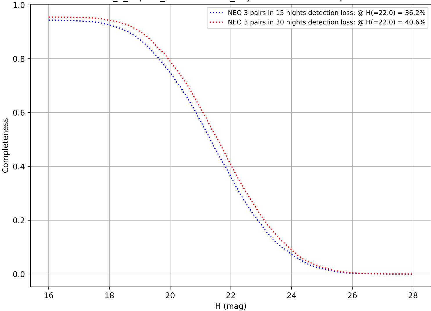
internal_u_expt30_nscale1.5v3.4_10yrs: DifferentialCompleteness
