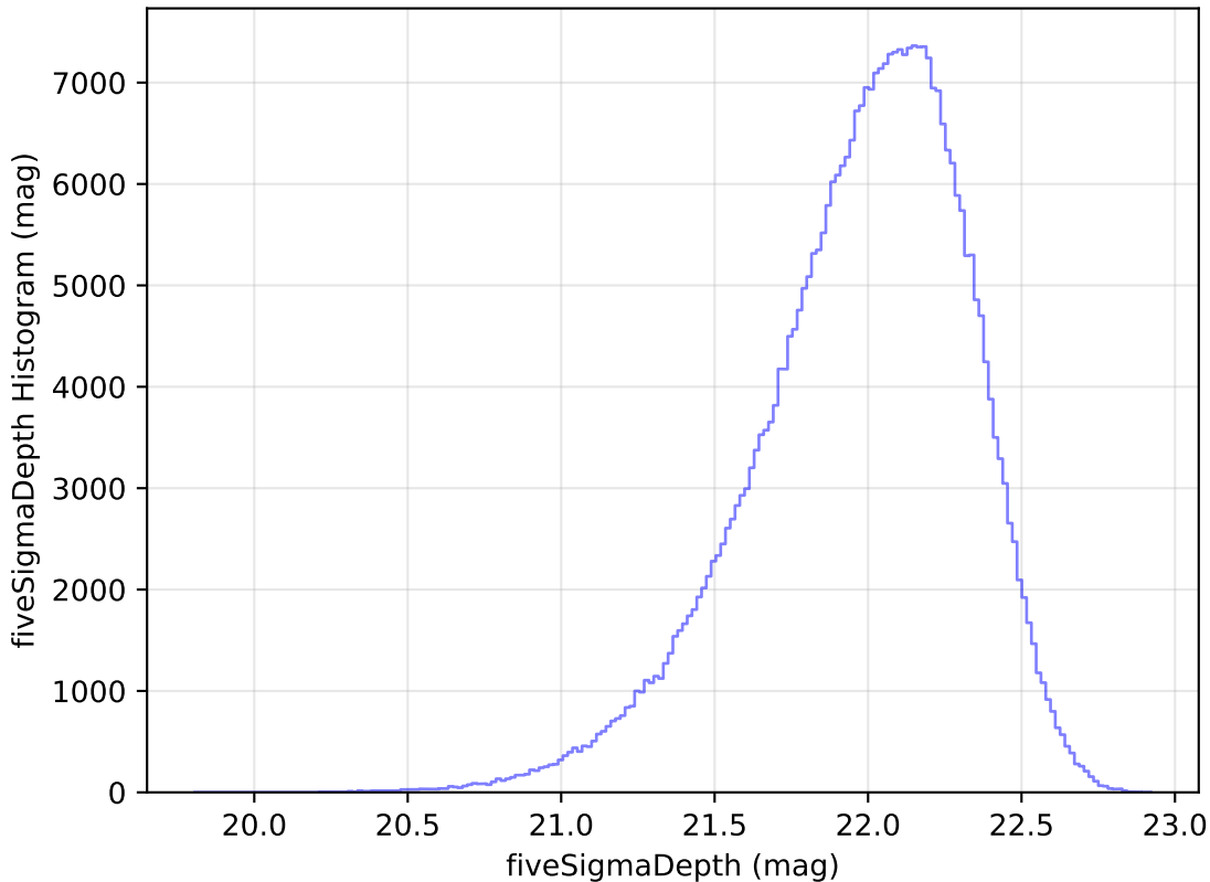
internal_u_expt30_nscale1.5v3.4_10yrs y: fiveSigmaDepth Histogram
