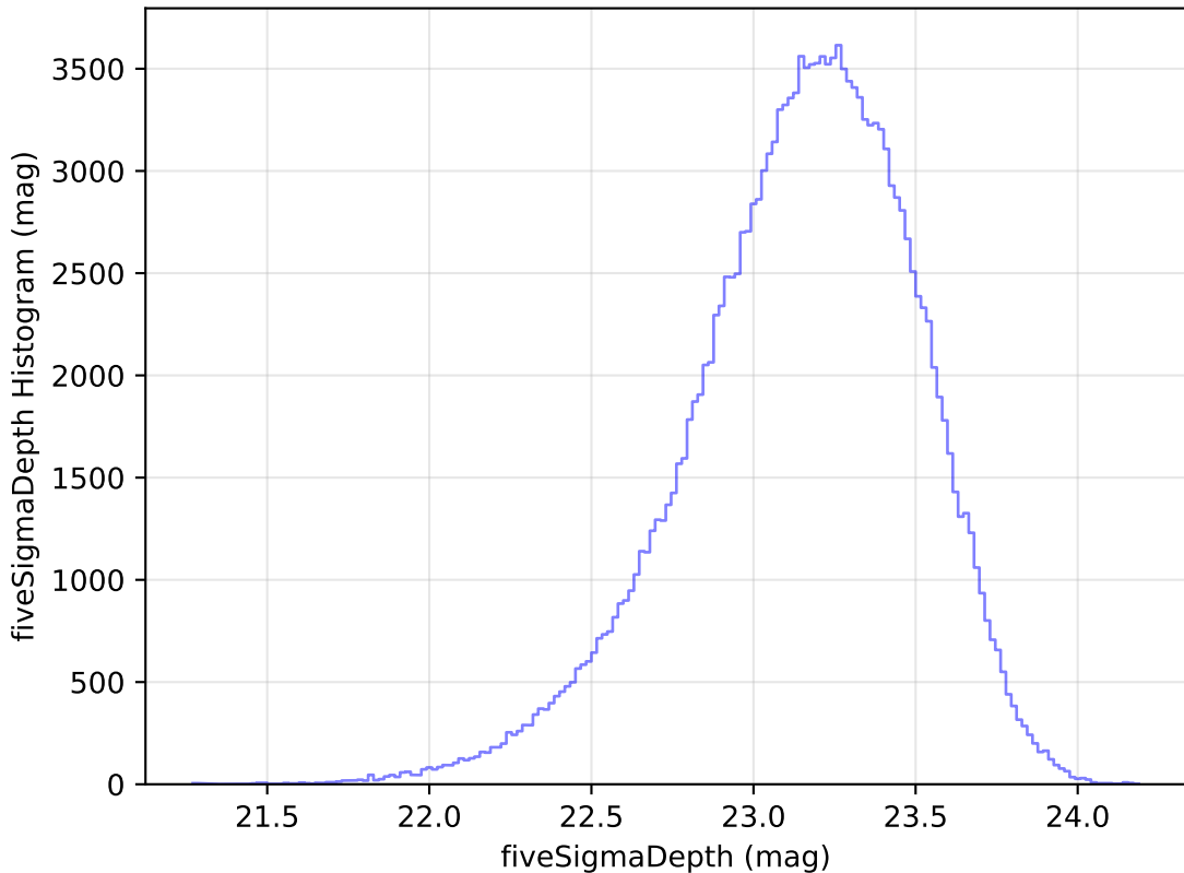
internal_u_expt30_nscale1.5v3.4_10yrs u: fiveSigmaDepth Histogram
