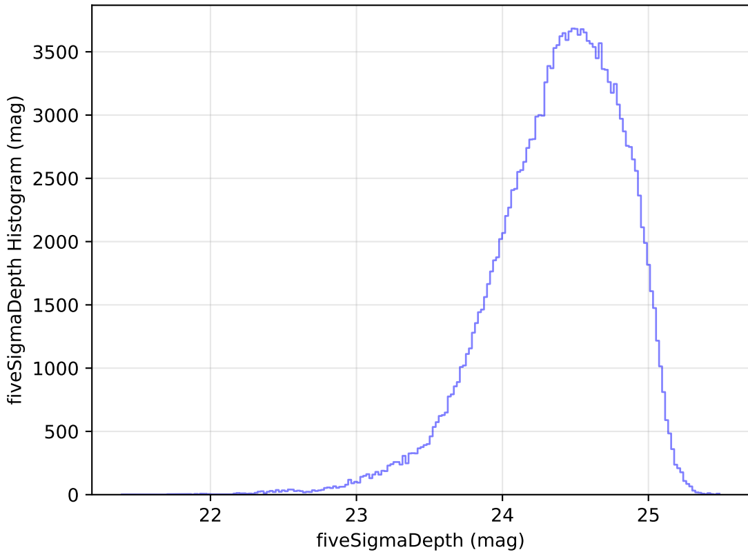
internal_u_expt30_nscale1.5v3.4_10yrs g: fiveSigmaDepth Histogram
