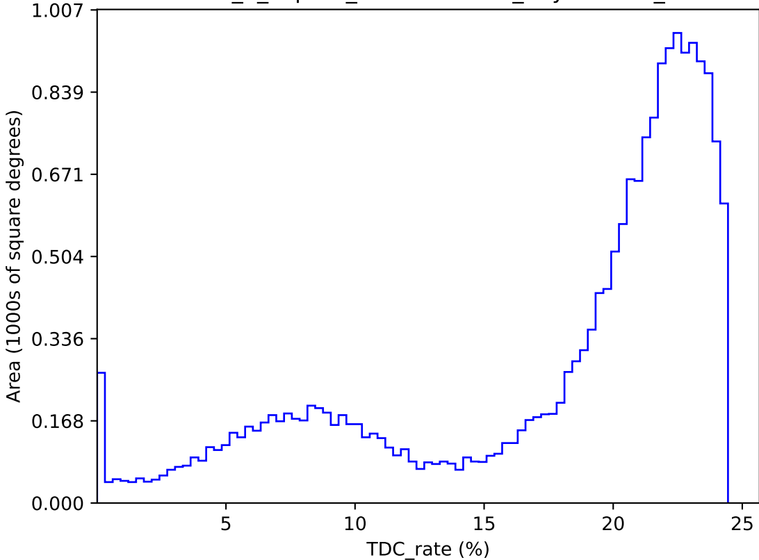
internal_u_expt30_nscale1.5v3.4_10yrs : TDC_rate
