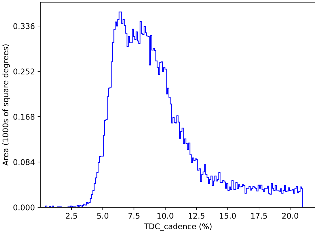
internal_u_expt30_nscale1.5v3.4_10yrs : TDC_cadence
