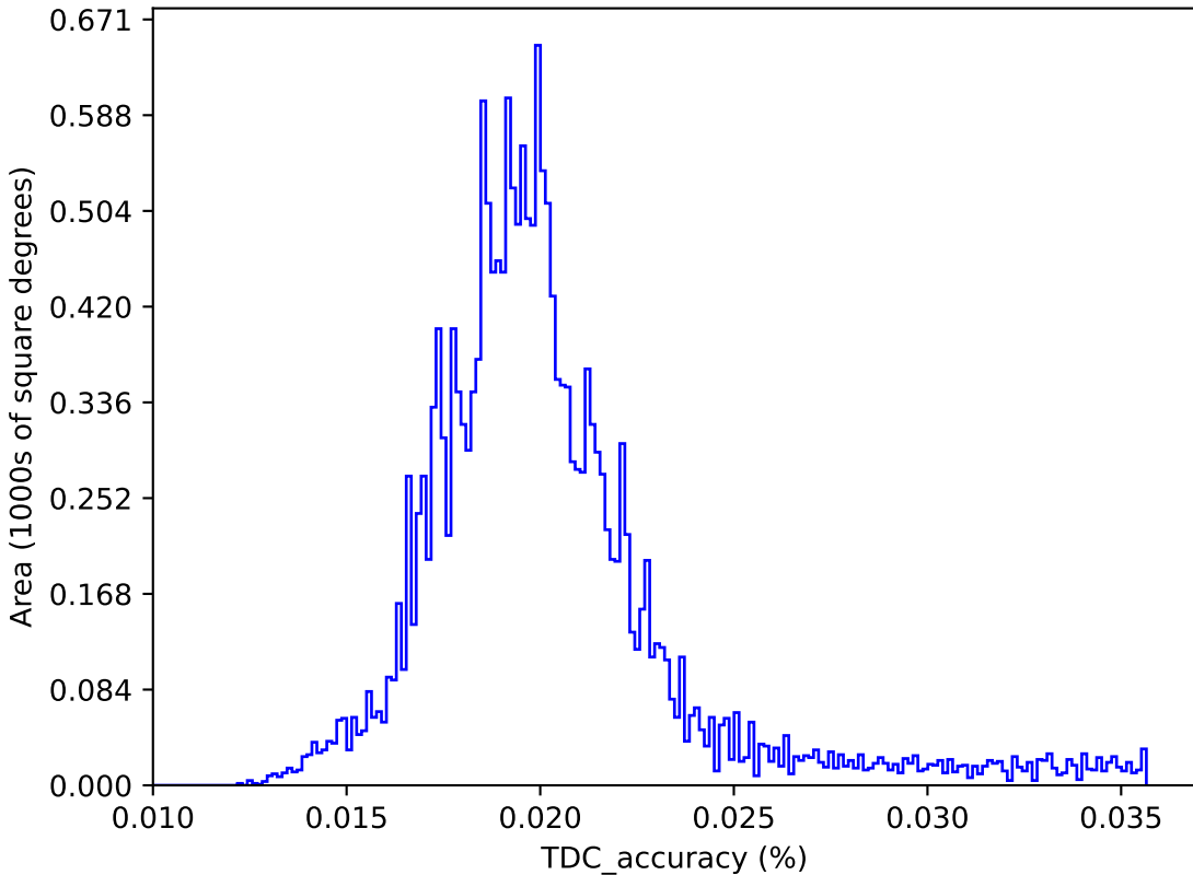
internal_u_expt30_nscale1.5v3.4_10yrs : TDC_accuracy
