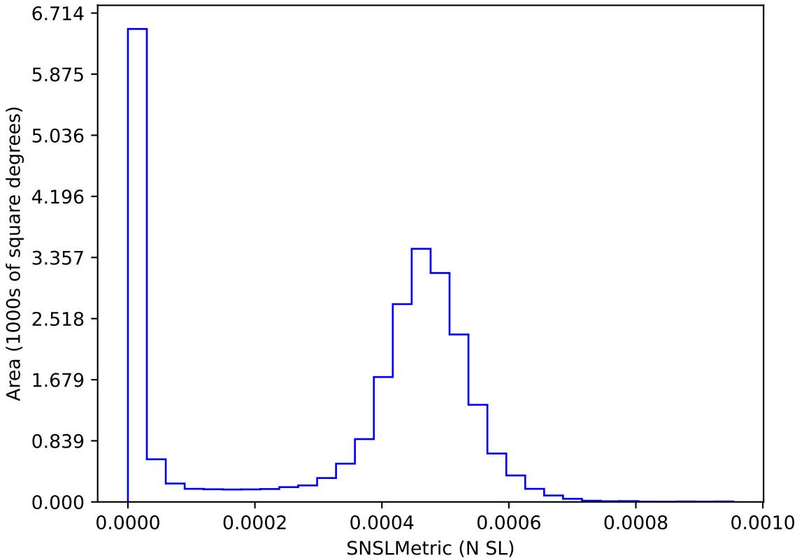
internal_u_expt30_nscale1.5v3.4_10yrs : SNSLMetric
