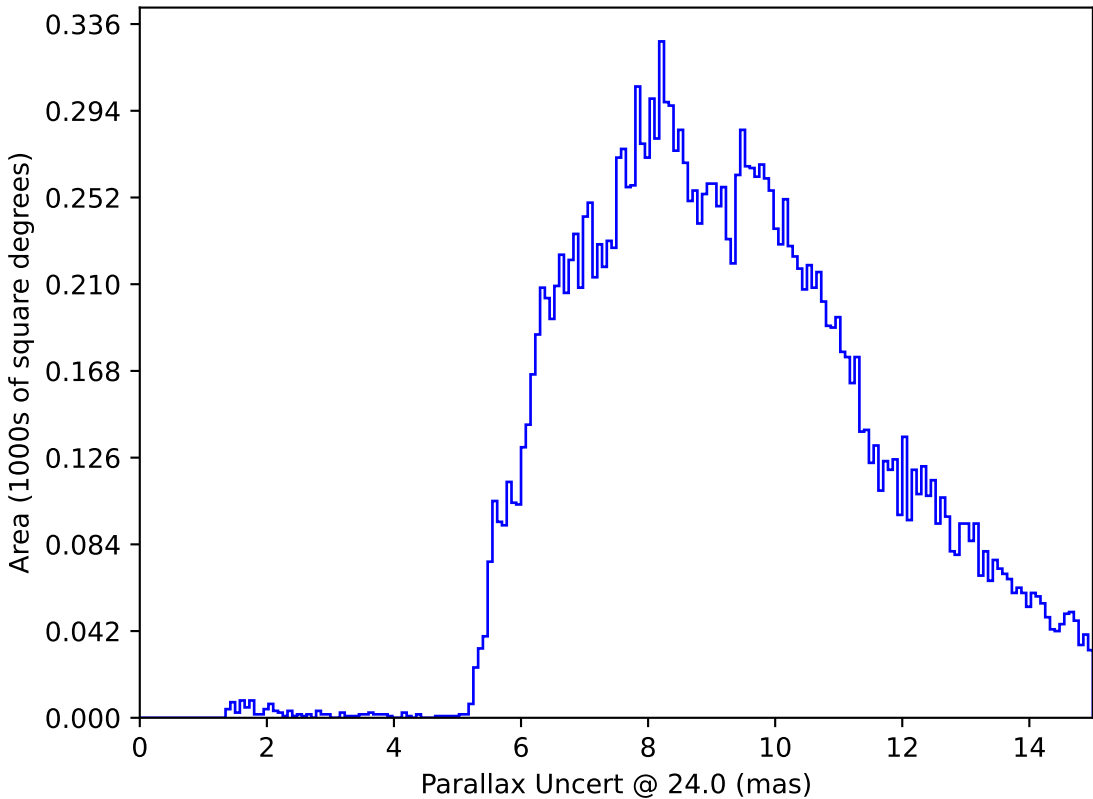
internal_u_expt30_nscale1.5v3.4_10yrs : Parallax Uncert @ 24.0
