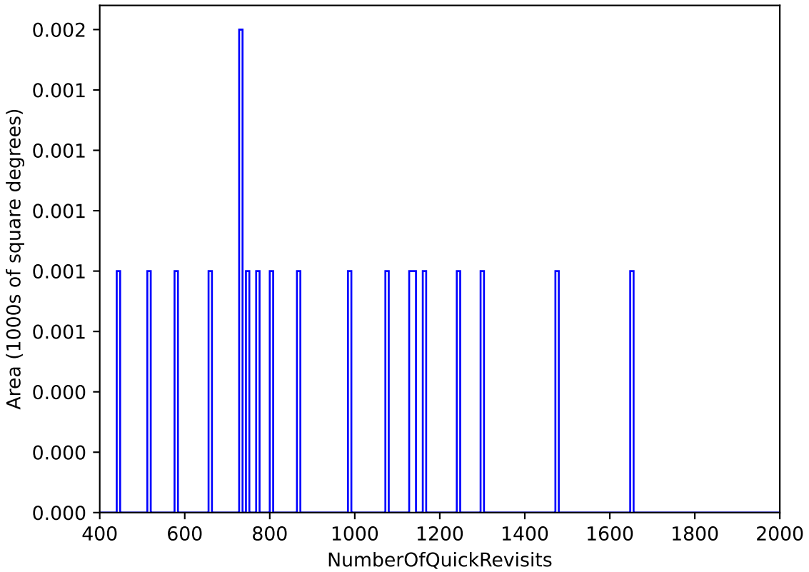
internal_u_expt30_nscale1.5v3.4_10yrs : NumberOfQuickRevisits
