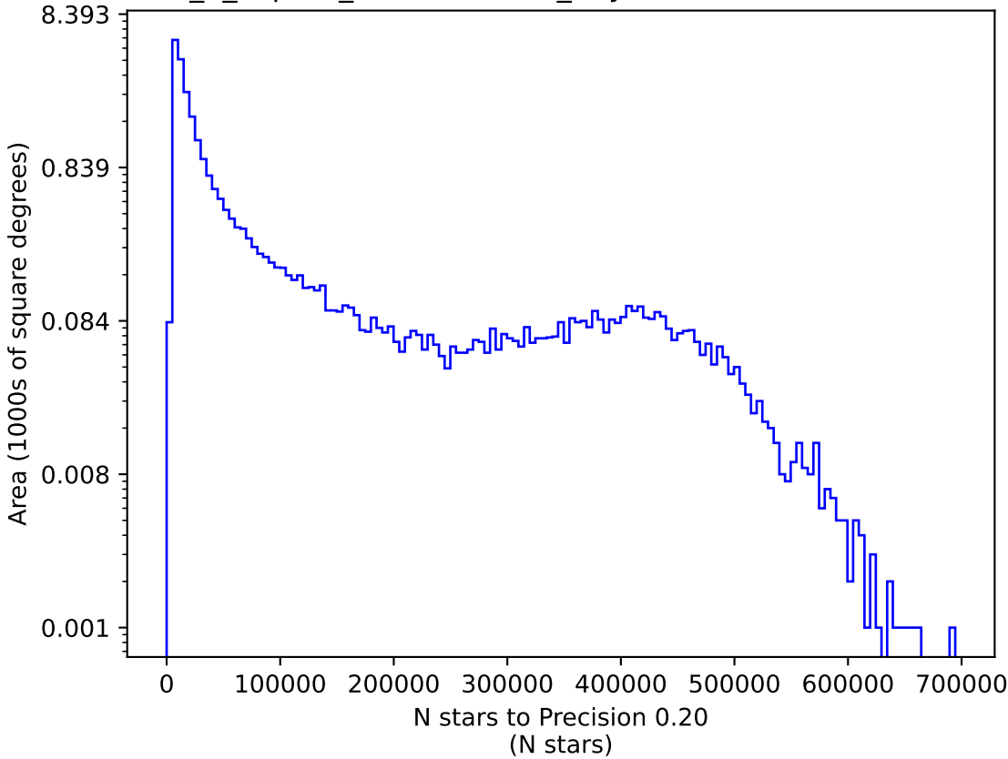
internal_u_expt30_nscale1.5v3.4_10yrs i: N stars to Precision 0.20
