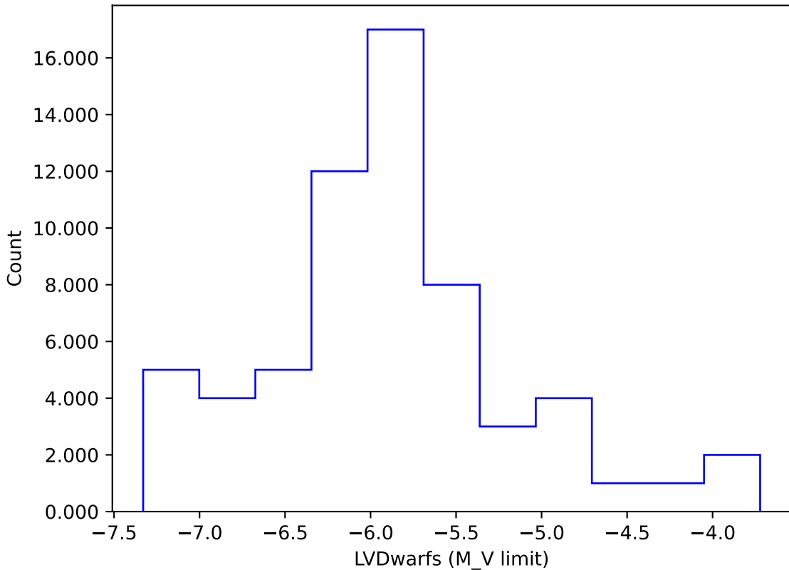
internal_u_expt30_nscale1.5v3.4_10yrs gi: LVDwarfs
