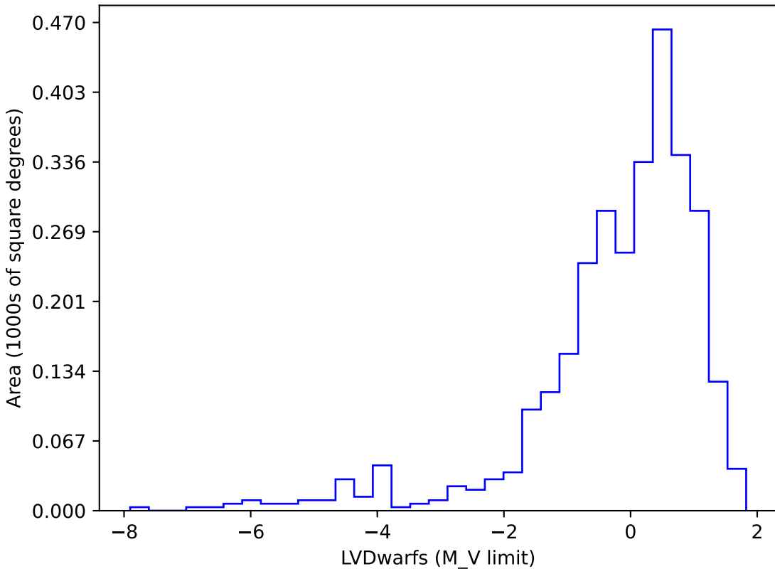
internal_u_expt30_nscale1.5v3.4_10yrs gi SCP: LVDwarfs
