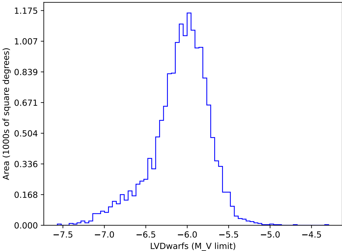
internal_u_expt30_nscale1.5v3.4_10yrs gi: LVDwarfs
