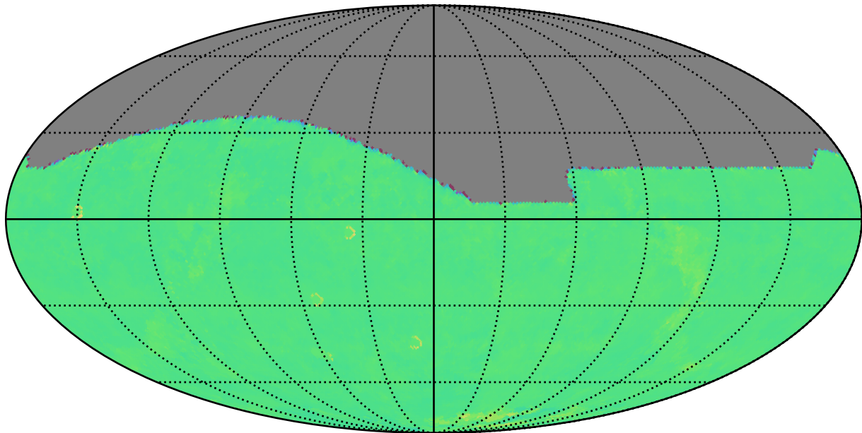
internal_u_expt30_nscale1.5v3.4_10yrs r: Kuiper rotTelPos
