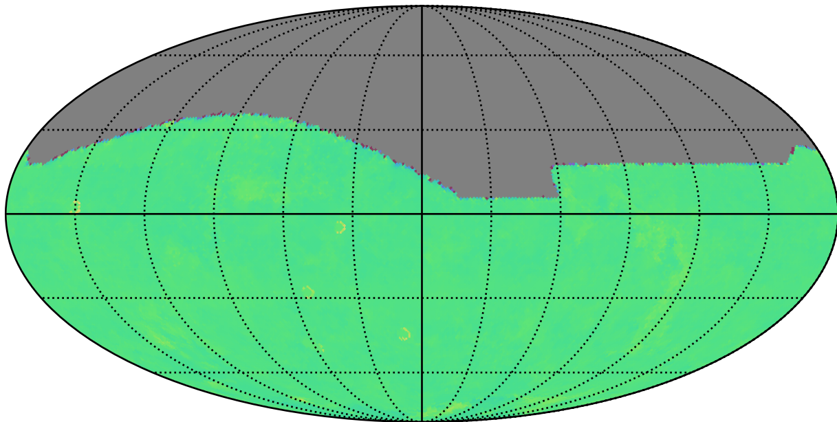
internal_u_expt30_nscale1.5v3.4_10yrs i: Kuiper rotTelPos
