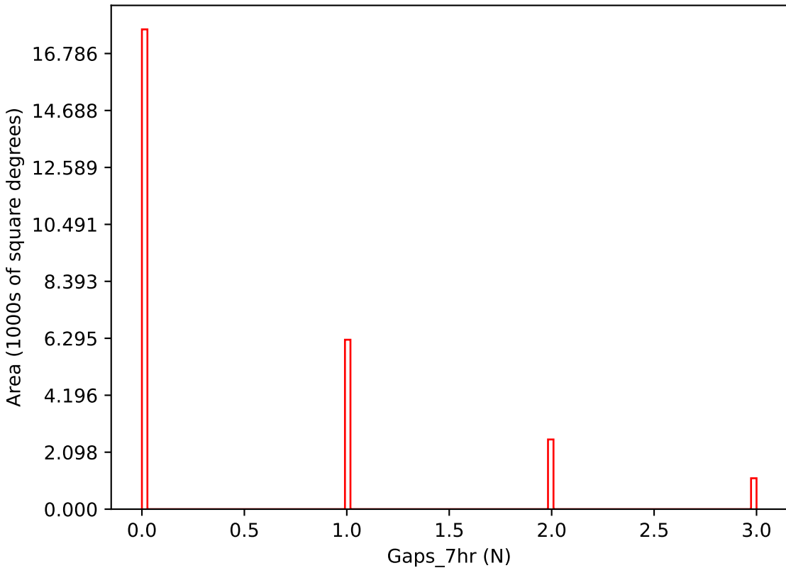
internal_u_expt30_nscale1.5v3.4_10yrs i band: Gaps_7hr
