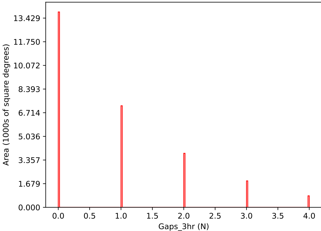
internal_u_expt30_nscale1.5v3.4_10yrs i band: Gaps_3hr
