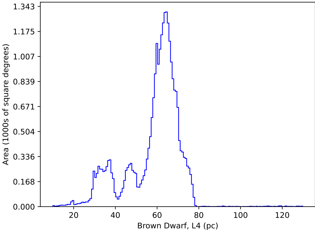
internal_u_expt30_nscale1.5v3.4_10yrs : Brown Dwarf, L4
