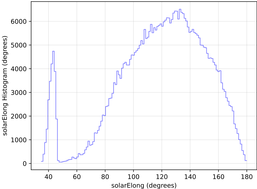
internal_u_expt30_nscale1.5v3.4_10yrs WFD z band: solarElong Histogram
