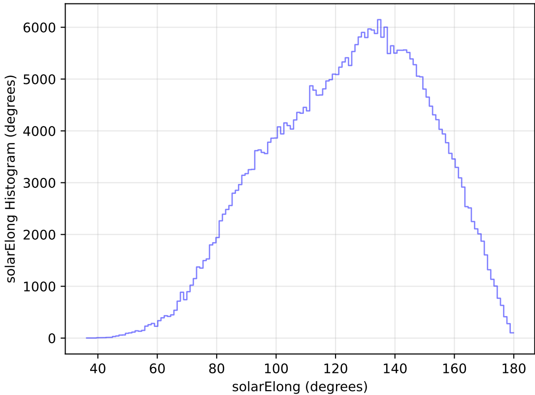
internal_u_expt30_nscale1.5v3.4_10yrs WFD y band: solarElong Histogram
