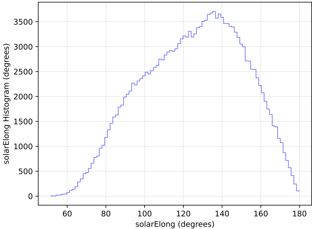
internal_u_expt30_nscale1.5v3.4_10yrs WFD u band: solarElong Histogram
