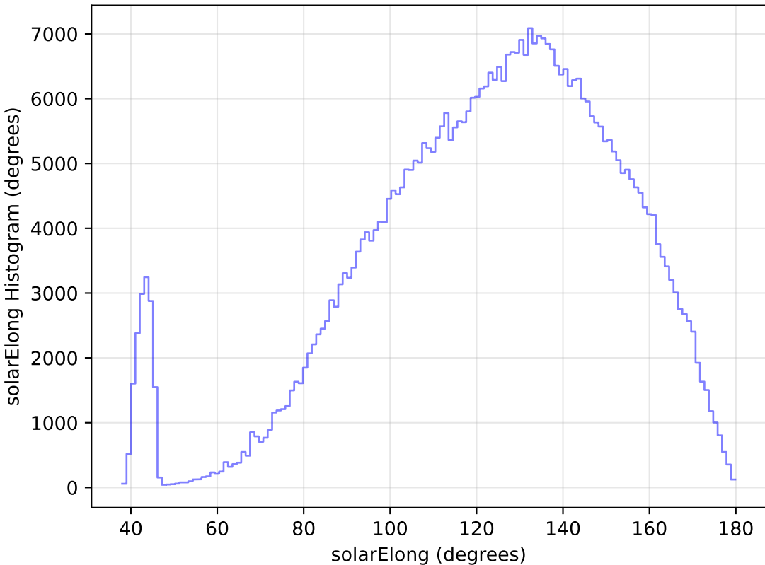
internal_u_expt30_nscale1.5v3.4_10yrs WFD r band: solarElong Histogram
