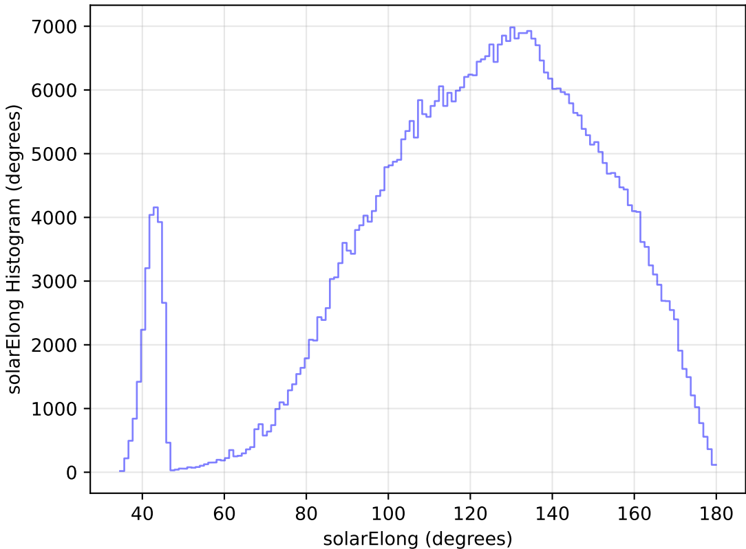
internal_u_expt30_nscale1.5v3.4_10yrs WFD i band: solarElong Histogram
