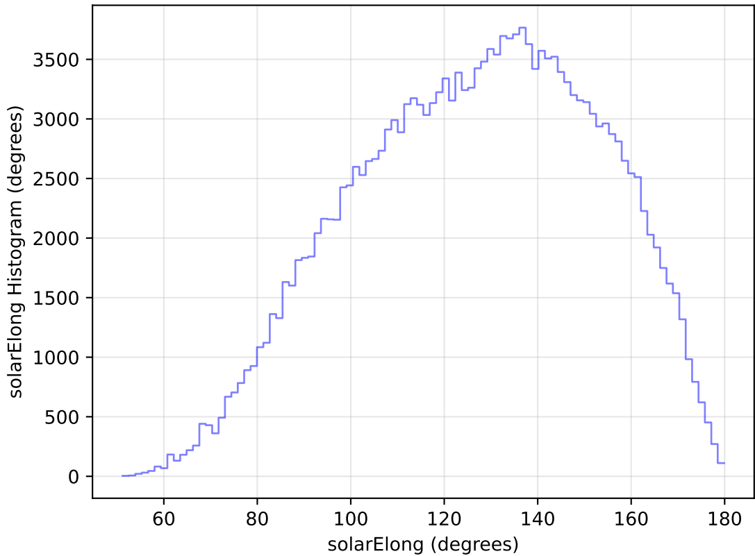
internal_u_expt30_nscale1.5v3.4_10yrs WFD g band: solarElong Histogram
