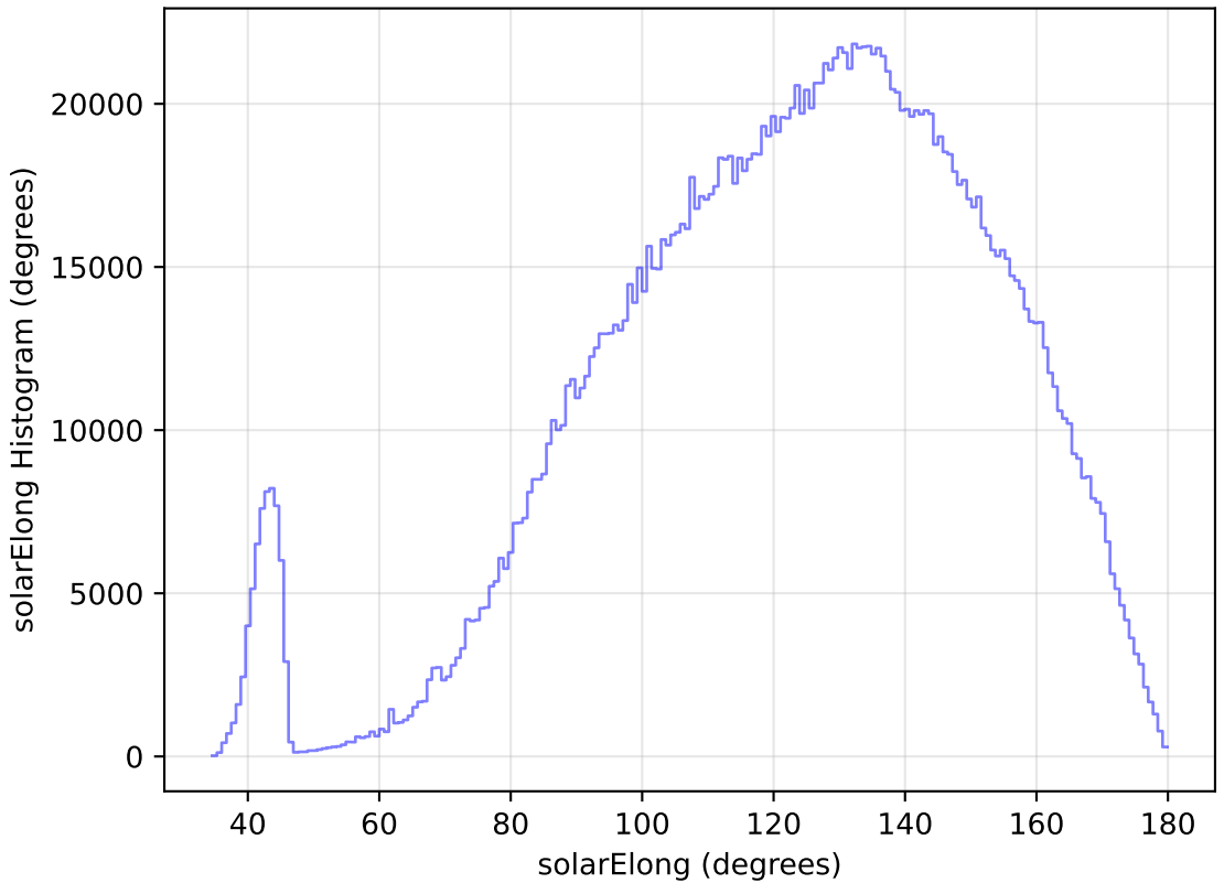
internal_u_expt30_nscale1.5v3.4_10yrs WFD all bands: solarElong Histogram
