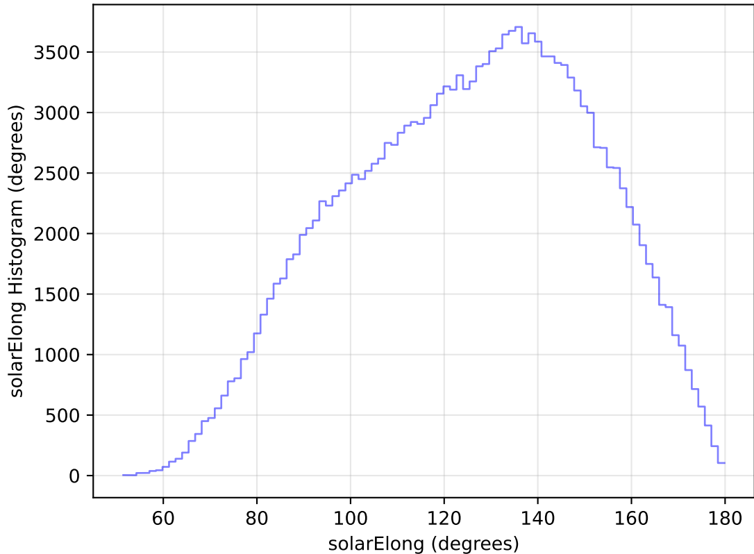
internal_u_expt30_nscale1.5v3.4_10yrs All sky u band: solarElong Histogram
