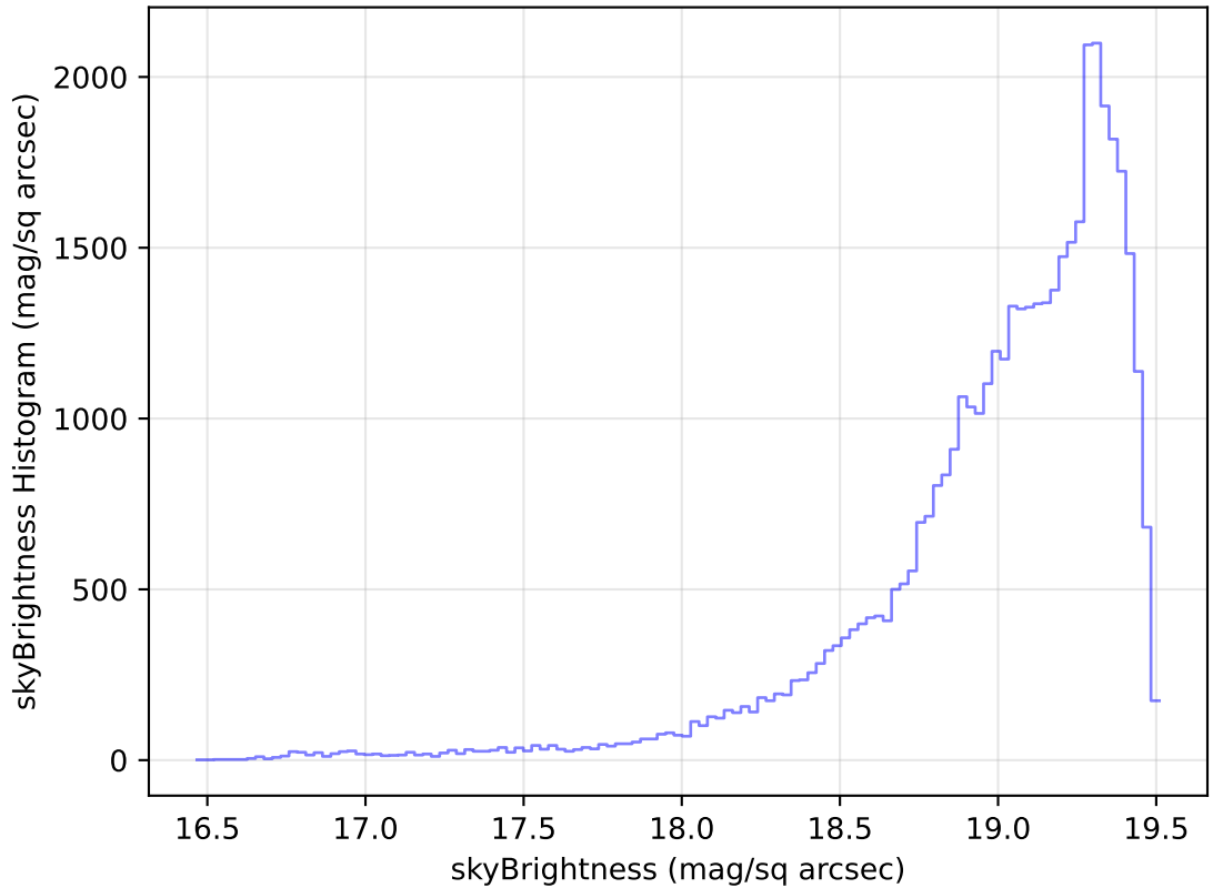
internal_u_expt30_nscale1.5v3.4_10yrs Yr 1 z band: skyBrightness Histogram
