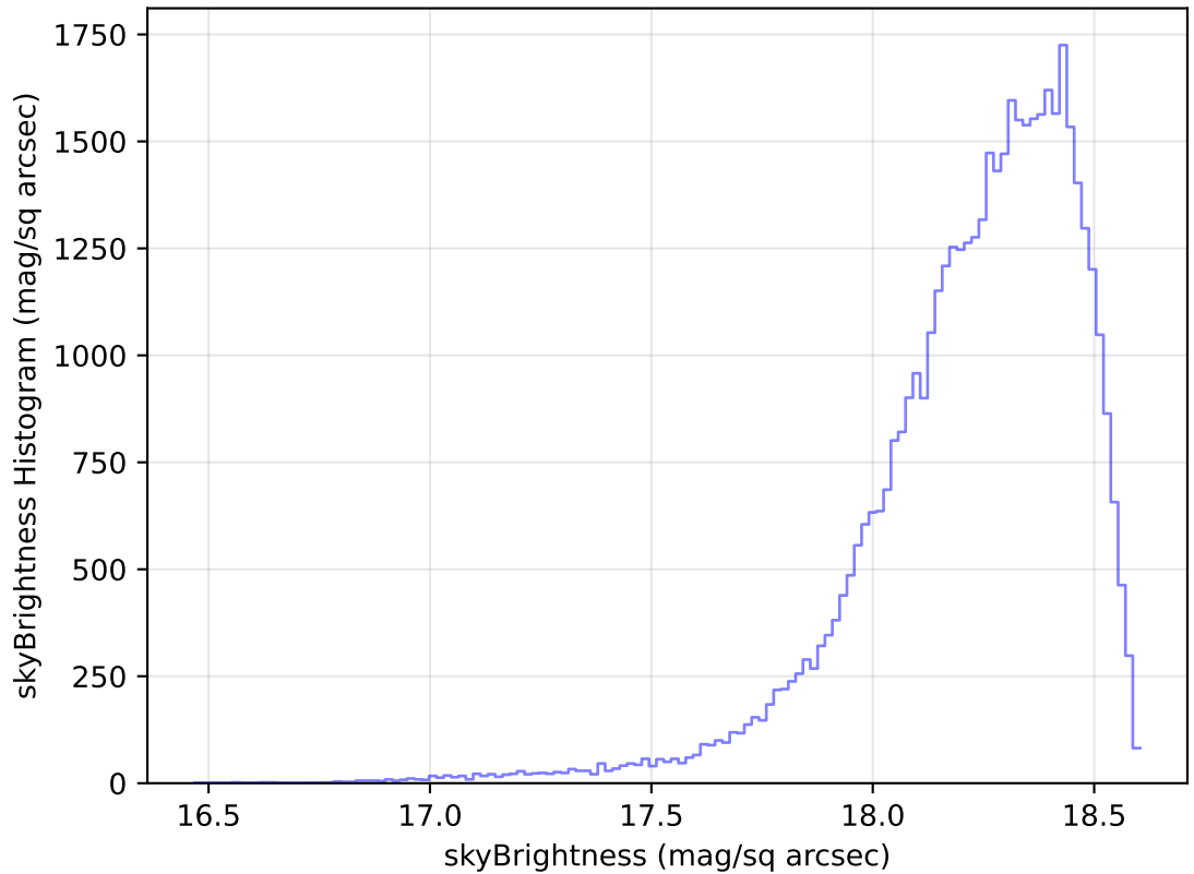
internal_u_expt30_nscale1.5v3.4_10yrs Yr 1 y band: skyBrightness Histogram
