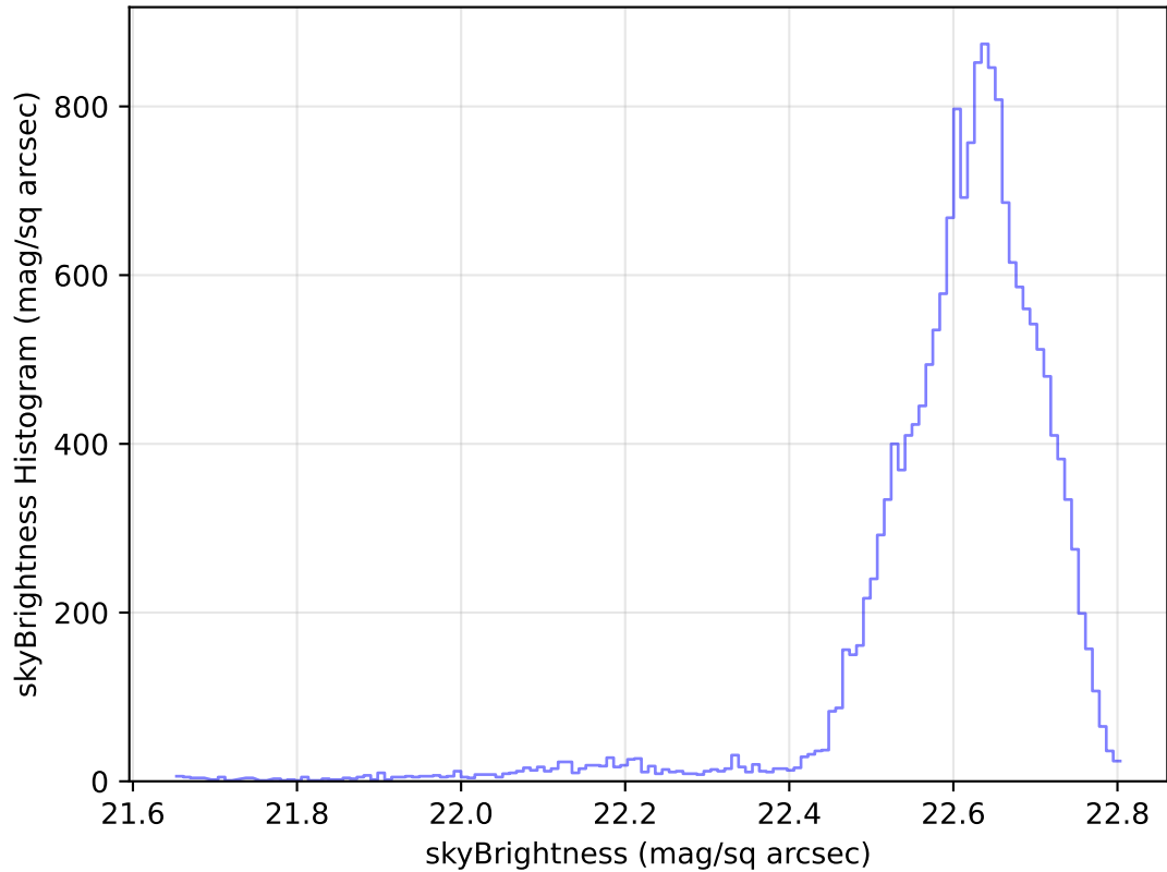
internal_u_expt30_nscale1.5v3.4_10yrs Yr 1 u band: skyBrightness Histogram
