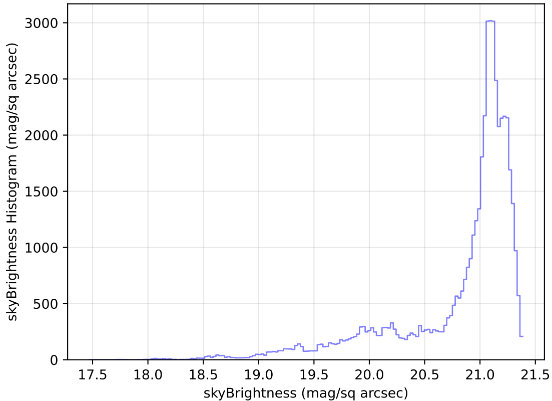
internal_u_expt30_nscale1.5v3.4_10yrs Yr 1 r band: skyBrightness Histogram
