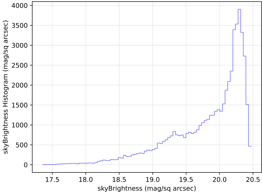
internal_u_expt30_nscale1.5v3.4_10yrs Yr 1 i band: skyBrightness Histogram
