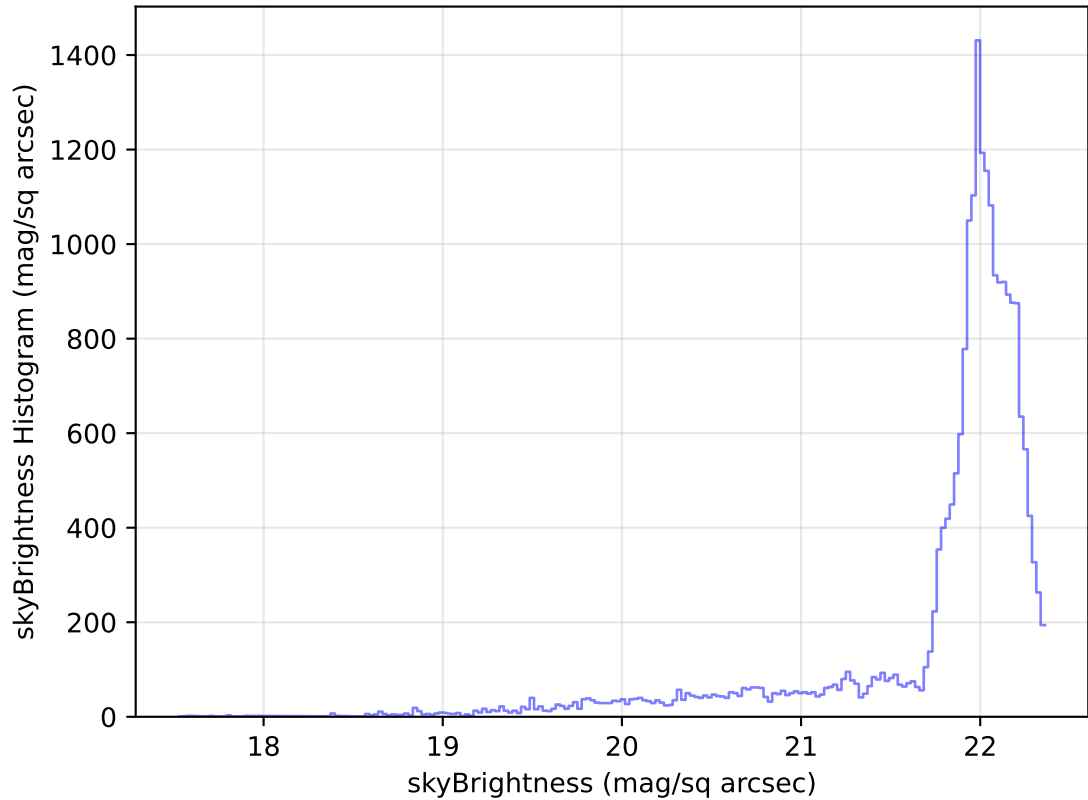
internal_u_expt30_nscale1.5v3.4_10yrs Yr 1 g band: skyBrightness Histogram
