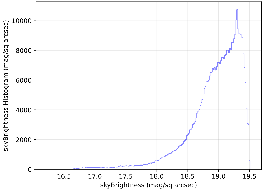
internal_u_expt30_nscale1.5v3.4_10yrs WFD z band: skyBrightness Histogram
