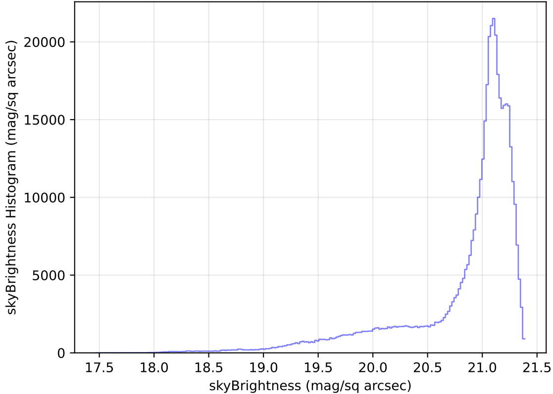
internal_u_expt30_nscale1.5v3.4_10yrs WFD r band: skyBrightness Histogram
