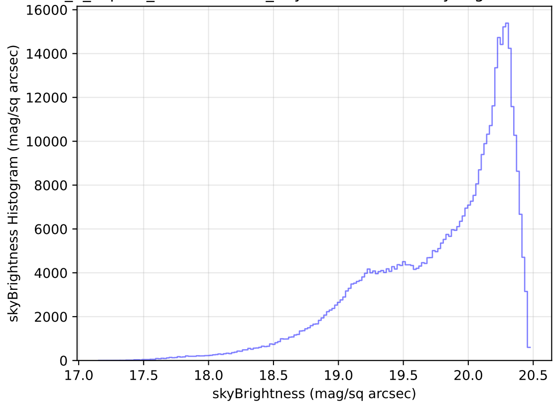
internal_u_expt30_nscale1.5v3.4_10yrs WFD i band: skyBrightness Histogram
