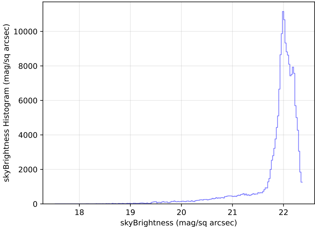
internal_u_expt30_nscale1.5v3.4_10yrs WFD g band: skyBrightness Histogram
