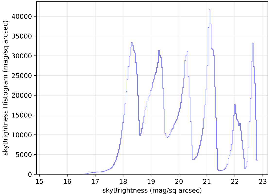
internal_u_expt30_nscale1.5v3.4_10yrs WFD all bands: skyBrightness Histogram
