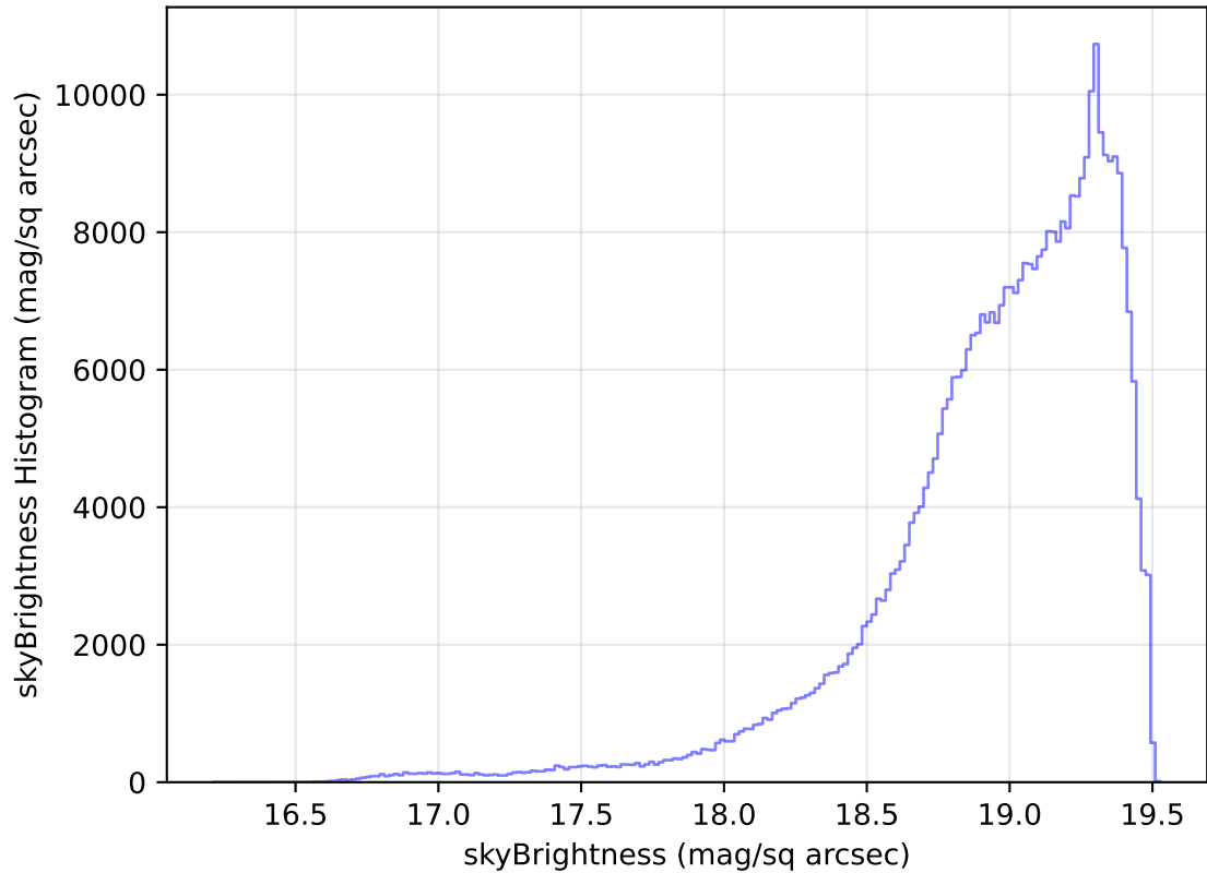
internal_u_expt30_nscale1.5v3.4_10yrs All sky z band: skyBrightness Histogram
