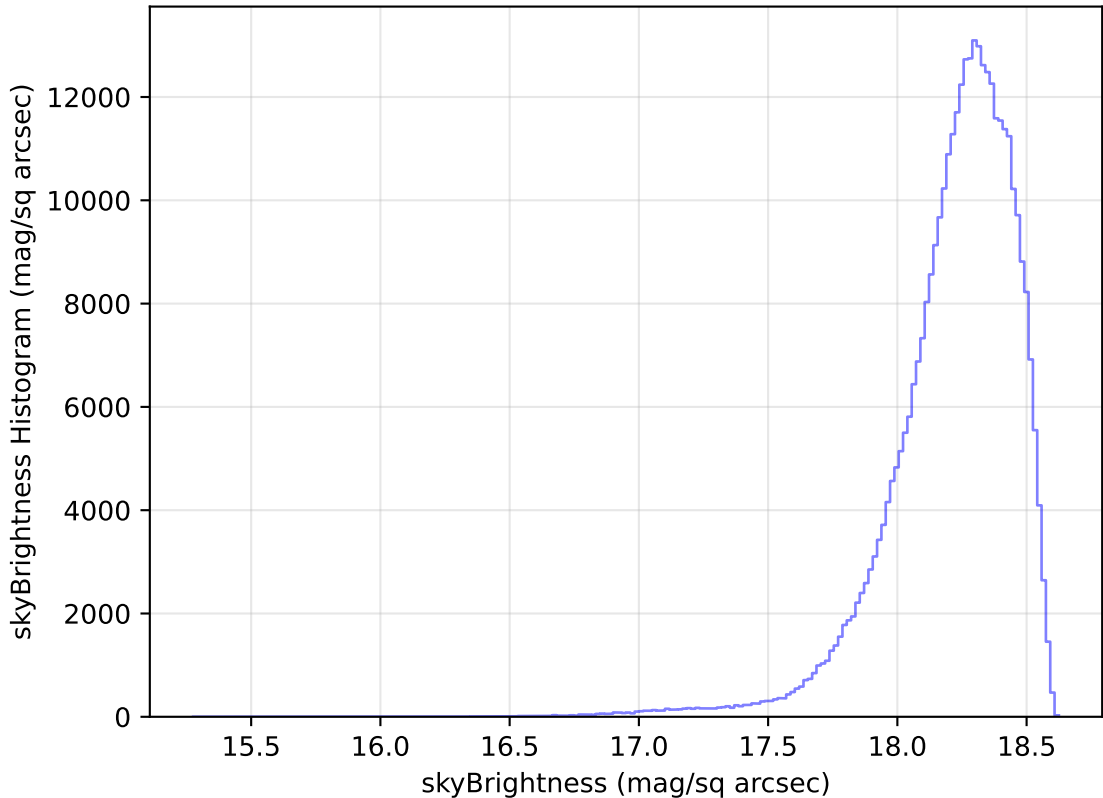
internal_u_expt30_nscale1.5v3.4_10yrs All sky y band: skyBrightness Histogram
