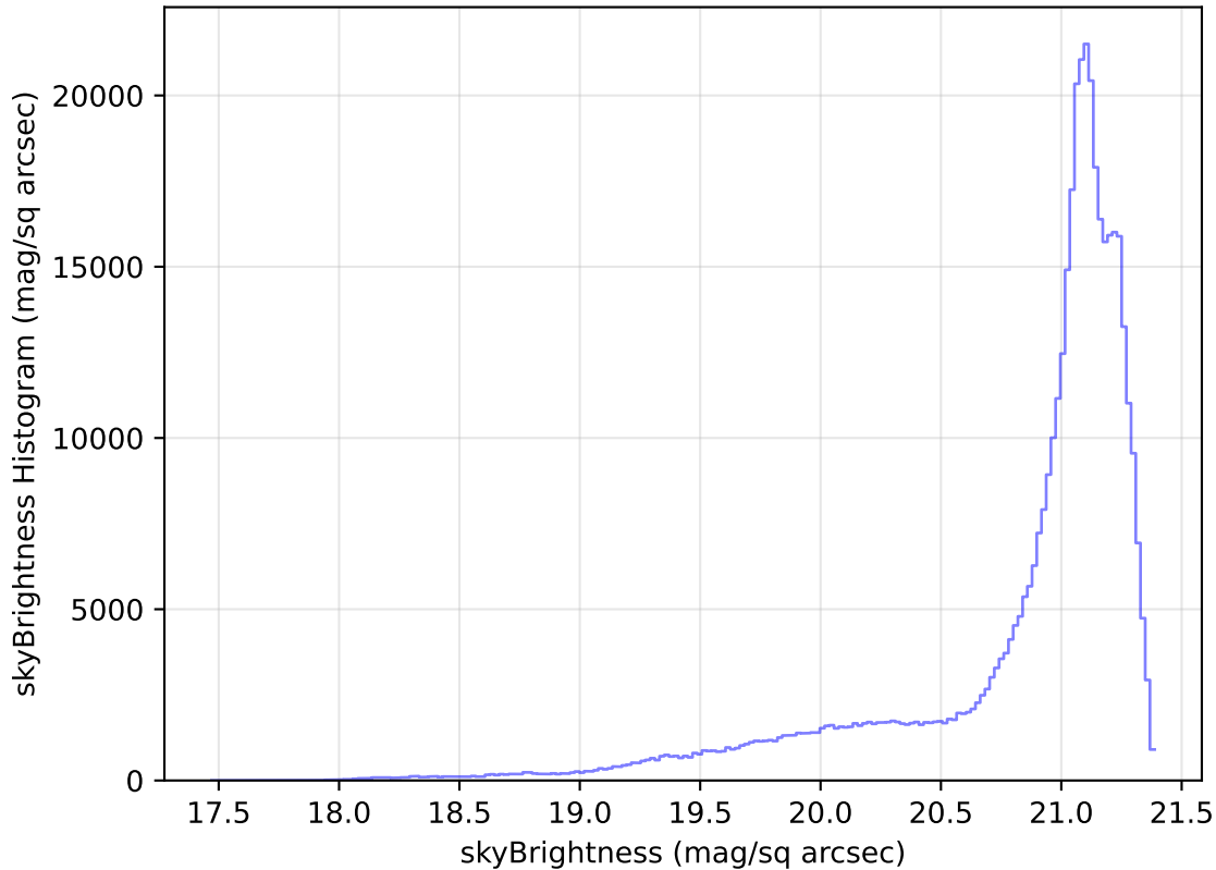
internal_u_expt30_nscale1.5v3.4_10yrs All sky r band: skyBrightness Histogram
